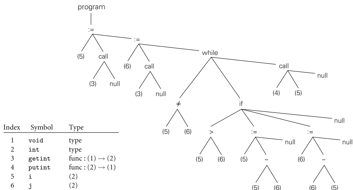
Figure 15.2 Syntax tree and symbol table for the GCD program. The only difference from Figure 1.6 is the addition of explicit null nodes to indicate empty argument lists and to terminate statement lists.
