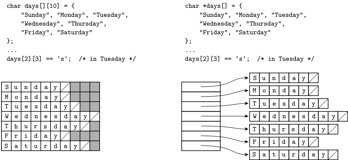
Figure 8.9 Contiguous array allocation vs row pointers in C. The declaration on the left is a true two-dimensional array. The slashed boxes are NUL bytes; the shaded areas are holes. The declaration on the right is a ragged array of pointers to arrays of characters. The arrays of characters may be located anywhere in memory—next to each other or separated, and in any order. In both cases, we have omitted bounds in the declaration that can be deduced from the size of the initializer (aggregate). Both data structures permit individual characters to be accessed using double subscripts, but the memory layout (and corresponding address arithmetic) is quite different.
