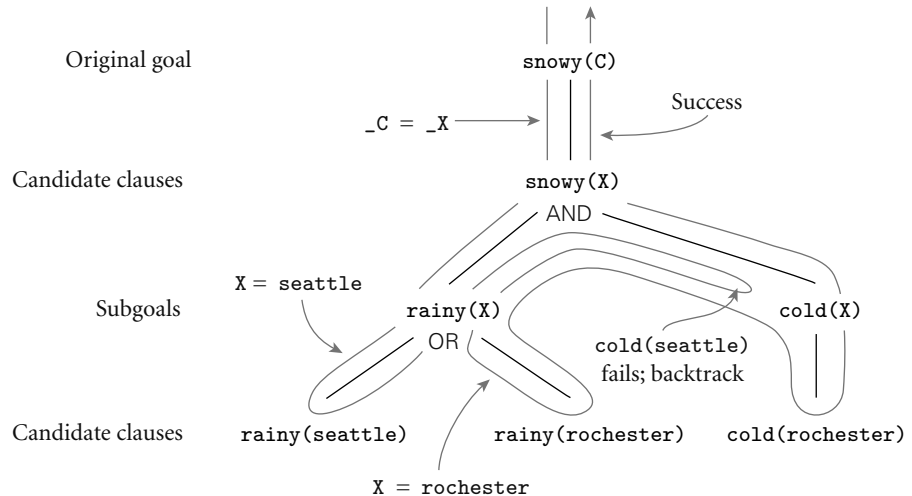
Figure 12.1 Backtracking search in Prolog. The tree of potential resolutions consists of alternating AND and OR levels. An AND level consists of subgoals from the right-hand side of a rule, all of which must be satisfied. An OR level consists of alternative database clauses whose head will unify with the subgoal above; one of these must be satisfied. The notation _C = _X is meant to indicate that while both C and X are uninstantiated, they have been associated with one another in such a way that if either receives a value in the future it will be shared by both.
