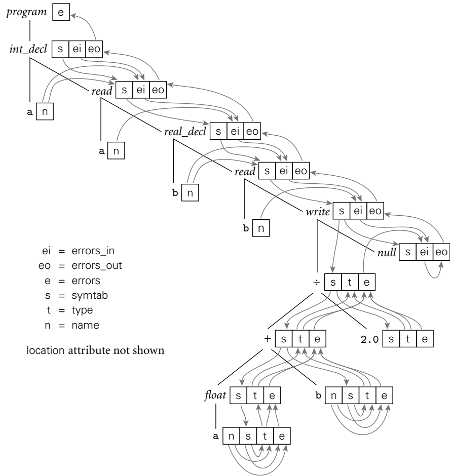
Figure 4.15 Decoration of the syntax tree of Figure 4.12, using the grammar of Figure 4.14.
