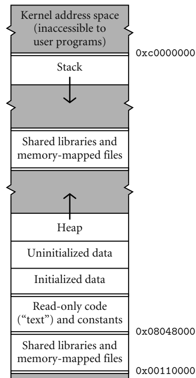
Figure 15.8 Layout of 32-bit process address space in x86 Linux (not to scale). Double lines separate regions with potentially different access permissions.
