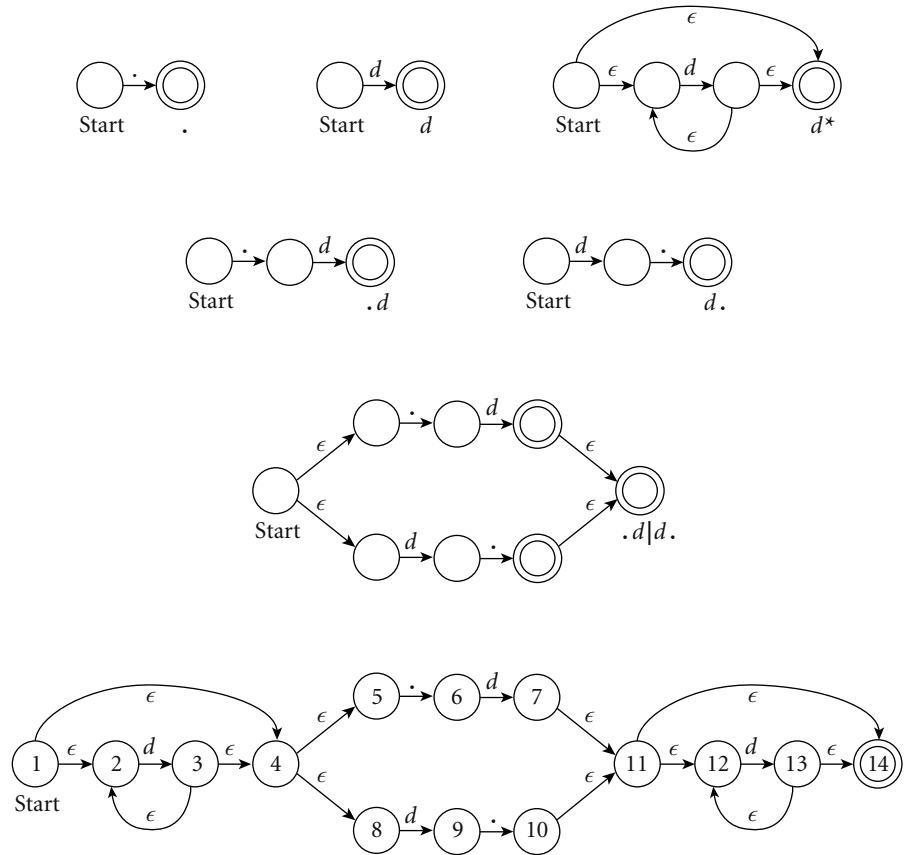
Figure 2.8 Construction of an NFA equivalent to the regular expression d^*(.d \mid d.)d^* . In the top row are the primitive automata for . and d , and the Kleene closure construction for d^* . In the second and third rows we have used the concatenation and alternation constructions to build .d , d. , and (.d \mid d.) . The fourth row uses concatenation again to complete the NFA. We have labeled the states in the final automaton for reference in subsequent figures.
