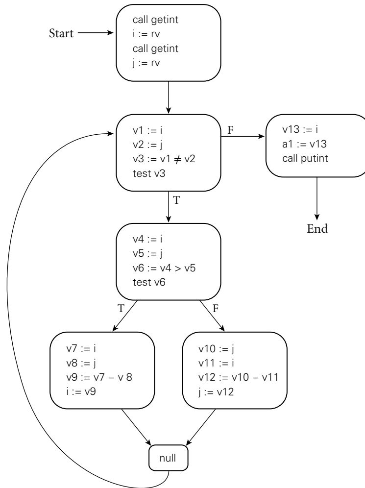
Figure 15.3 Control flow graph for the GCD program. Code within basic blocks is shown in the pseudo-assembly notation introduced in Sidebar 5.1, with a different virtual register (here named v1...v13) for every computed value. Registers a1 and rv are used to pass values to and from subroutines.
