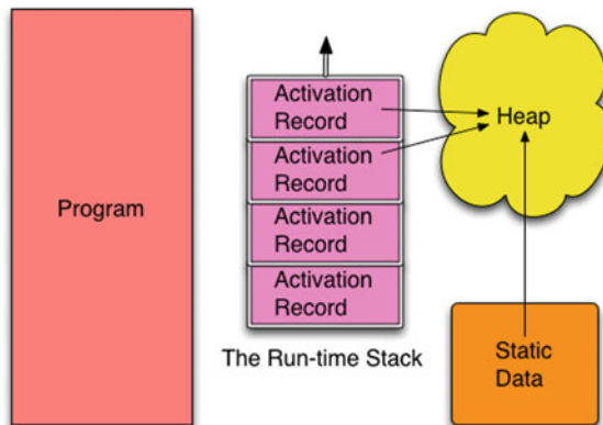
Fig. 1.4 Imperative model
