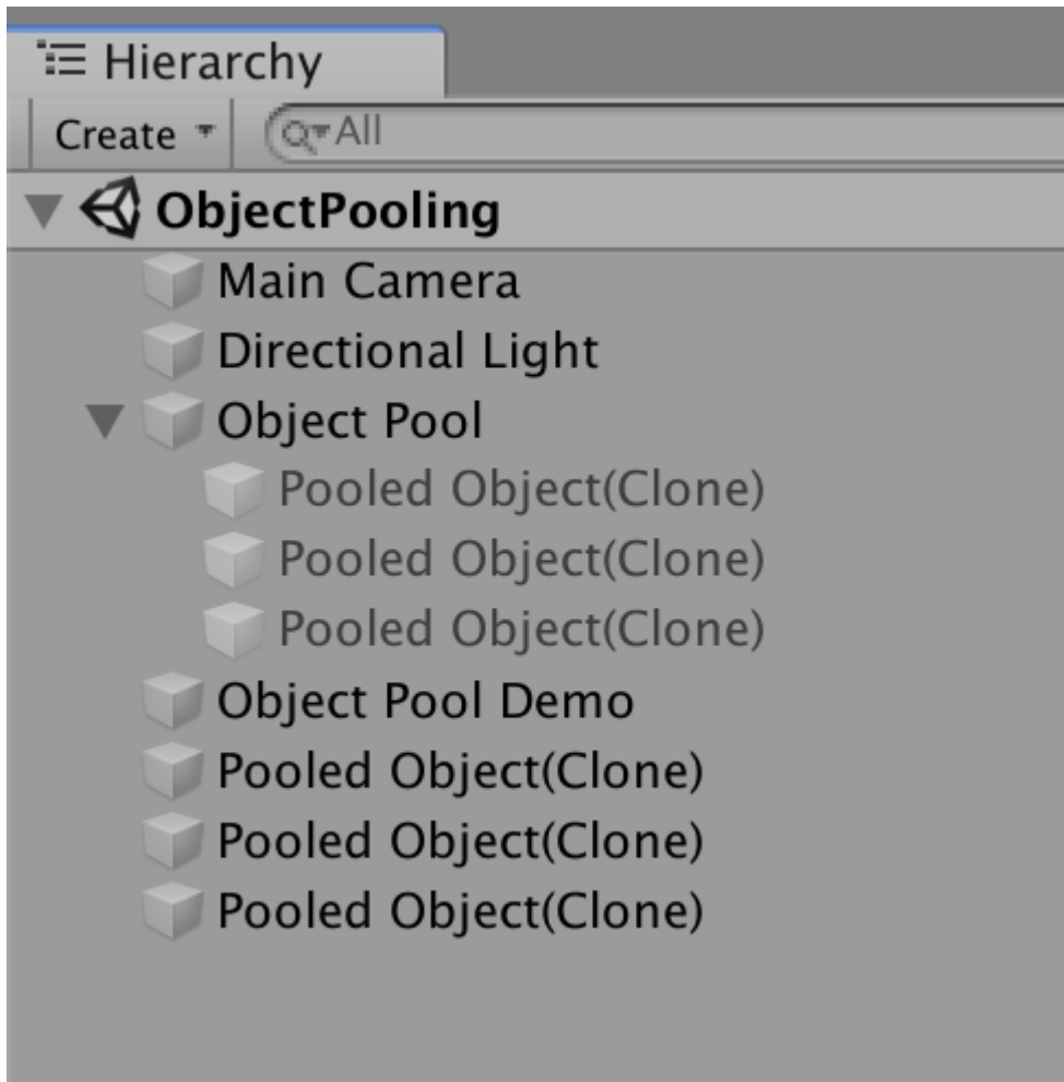
Figure 2-6. As objects return to the pool, they are disabled and temporarily made children of the object pool rather than being destroyed and having their memory freed.
