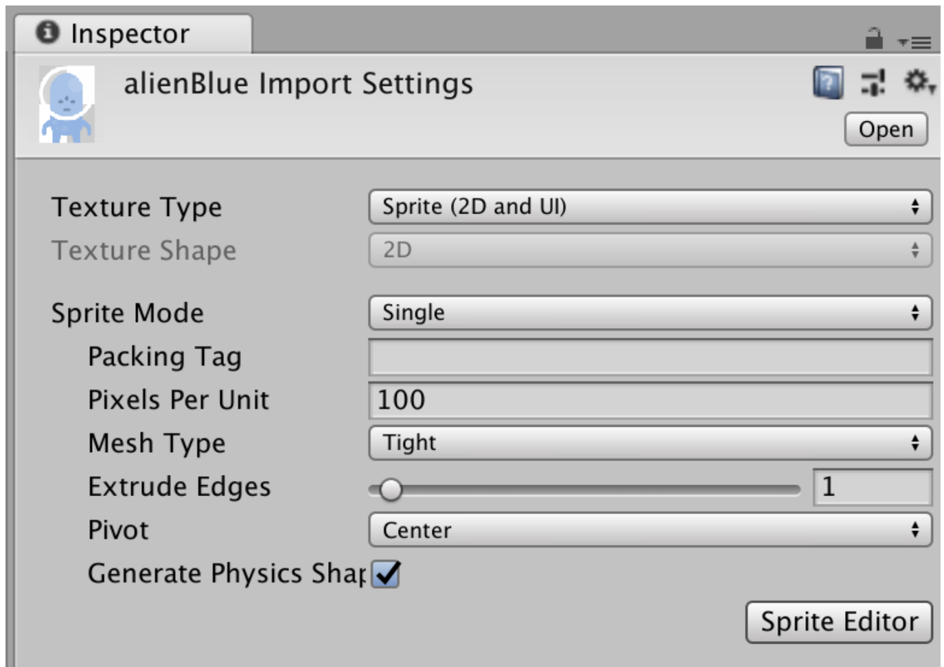
Figure 5-3. Enabling the Generate Physics Shape option in the import settings for a sprite texture.
