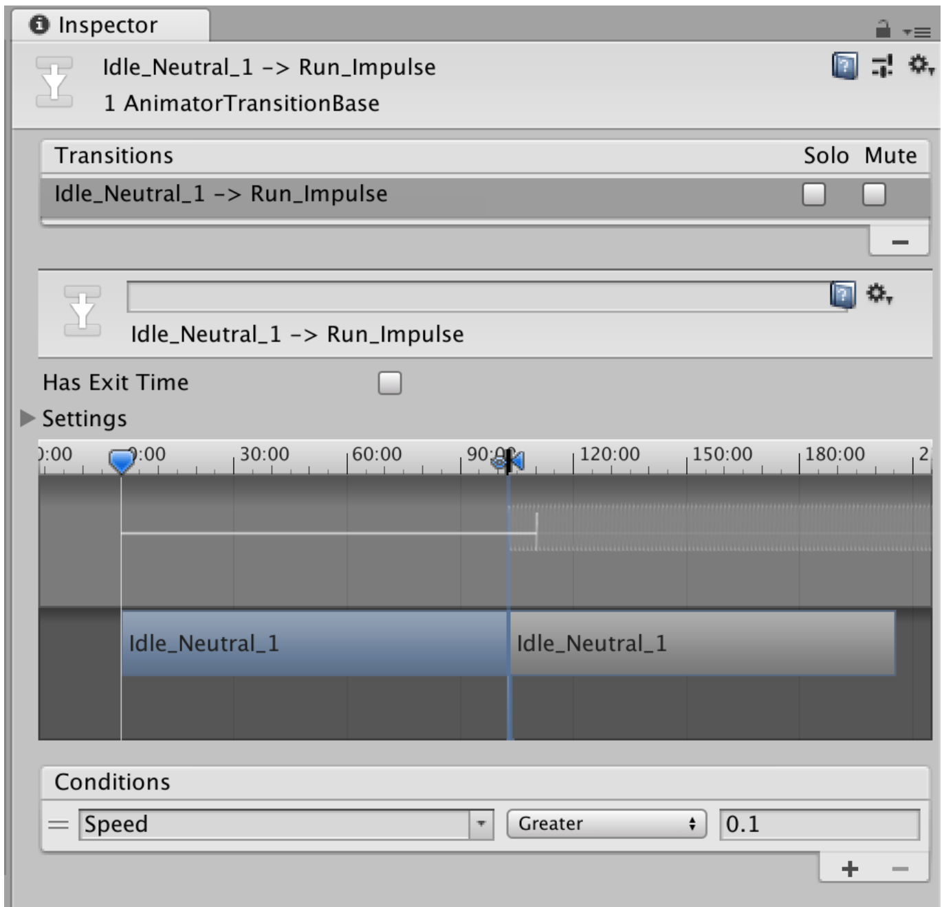
Figure 8-6. The settings for the transition from the Idle animation to the Run animation.
