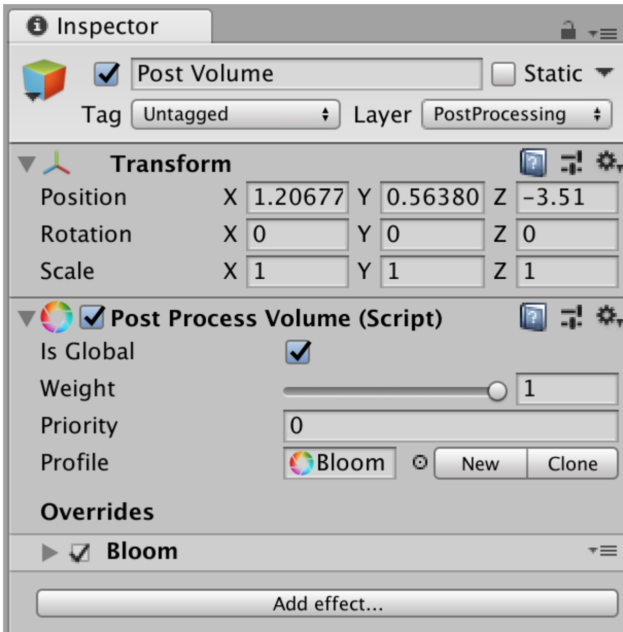
Figure 6-6. The Inspector for a Post-Processing volume game object. In addition to the Post-Processing Volume component, the game object's layer has been set to PostProcessing.
