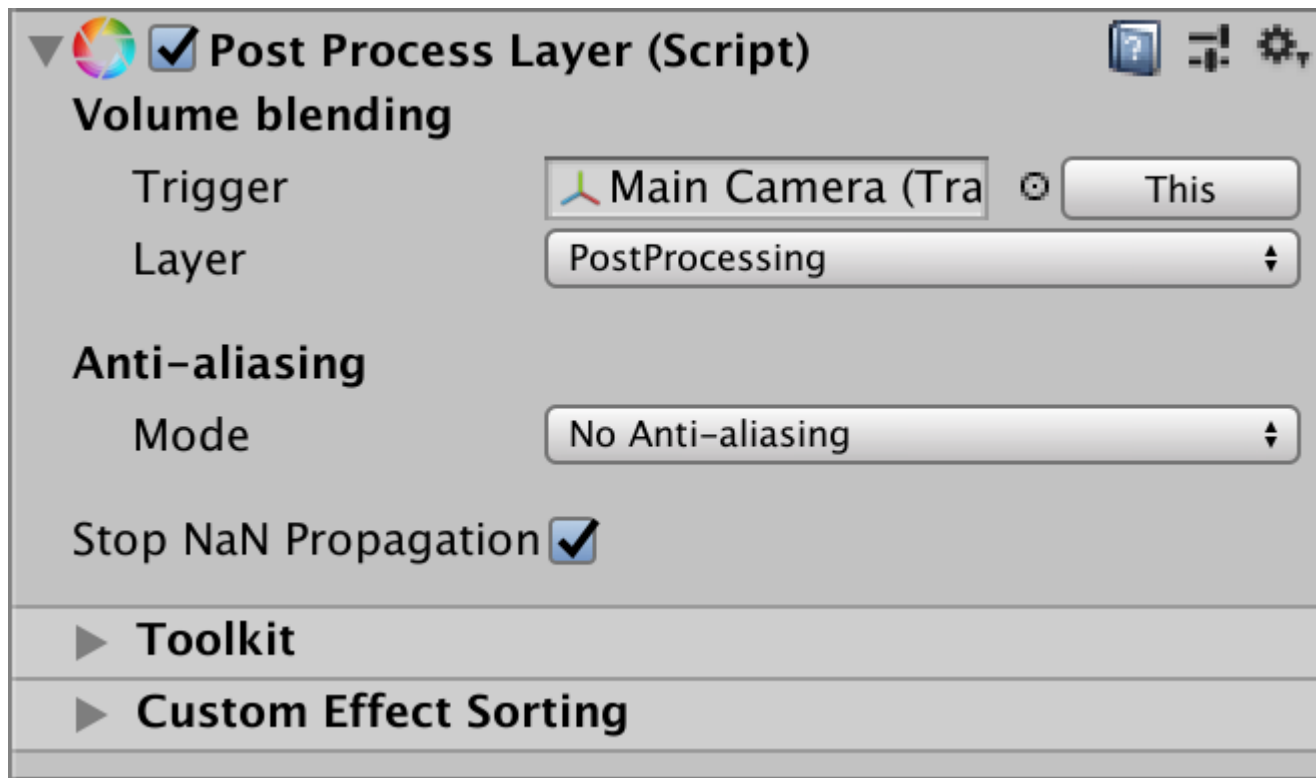
Figure 6-8. Configuring a Post Process Layer component to use the PostProcessing object layer.
