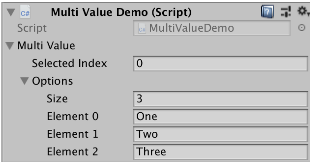
Figure 12-12. The Inspector for a MultiValue property.
