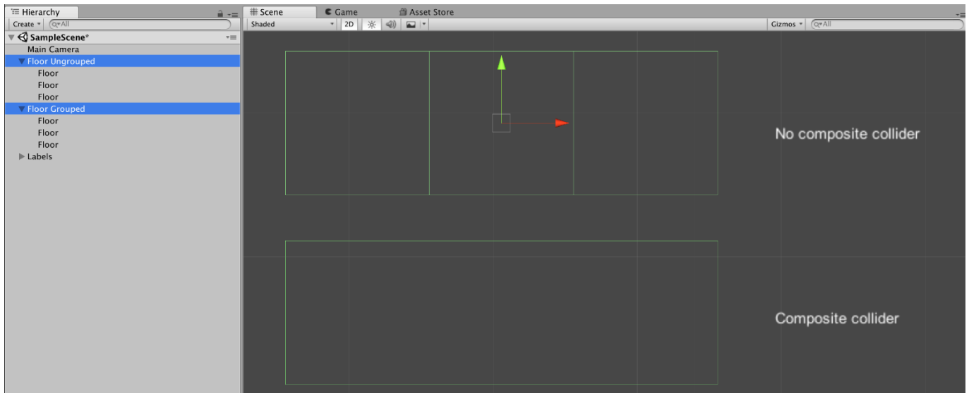
Figure 5-7. Two groups of colliders; the group at the top does not use a composite collider, and the individual outlines of the shapes can be seen. The group at the bottom does use a composite collider, and the shapes have been merged into a single outline.
