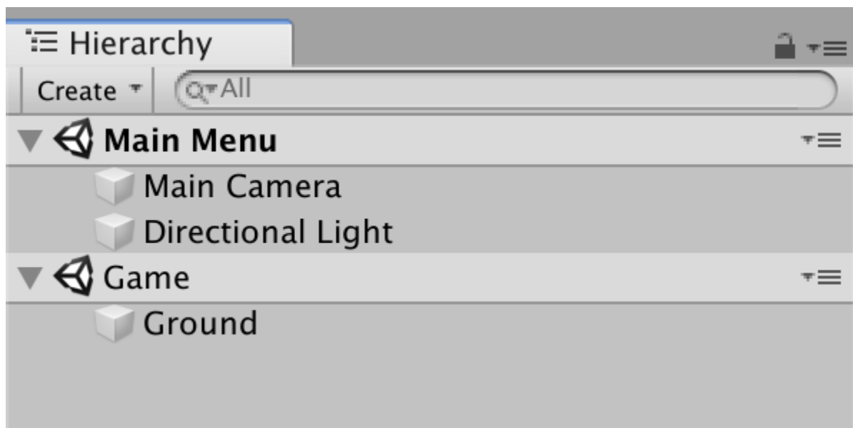
Figure 2-5. The Hierarchy tab, with two scenes loaded at the same time.
