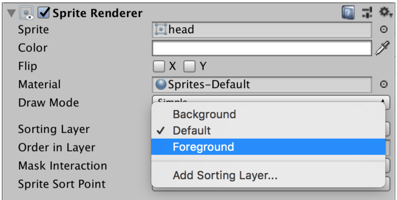
Figure 5-14. Selecting a sorting layer for a sprite renderer.
