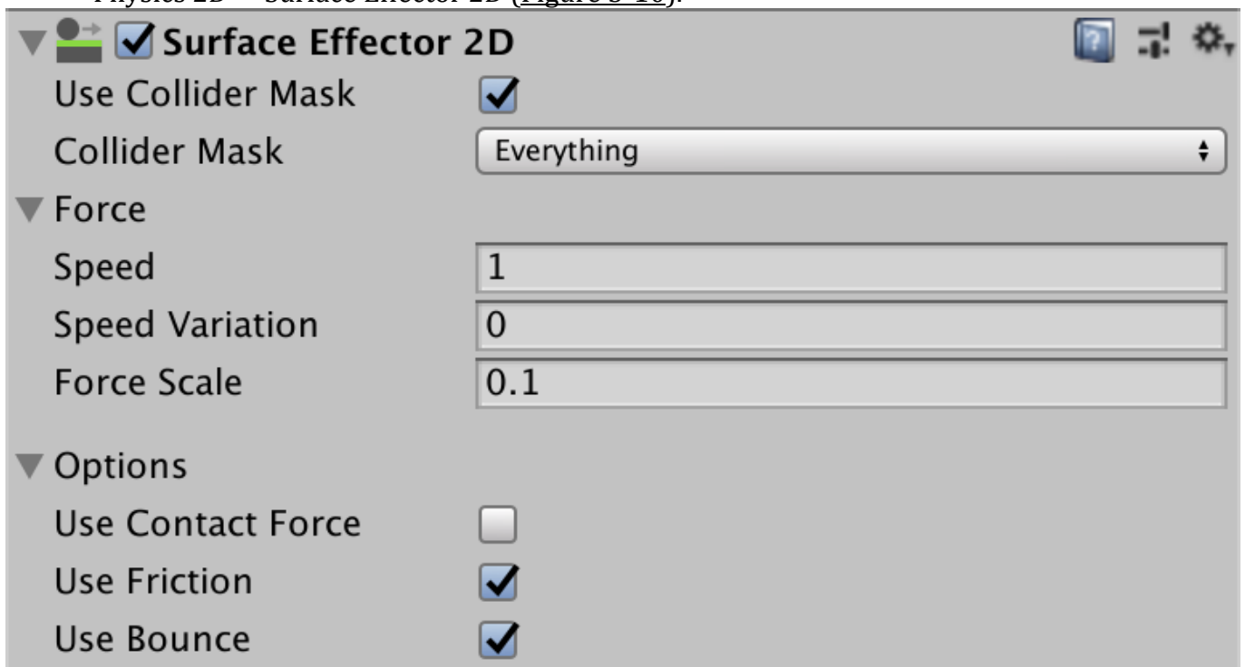
Figure 5-10. The settings of a SurfaceEffector2D component.
