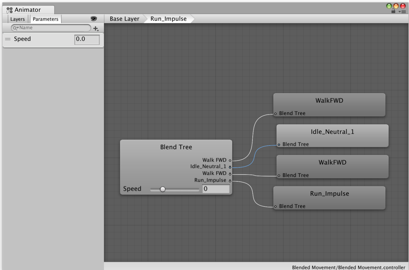
Figure 8-12. The blend tree for the four states.
