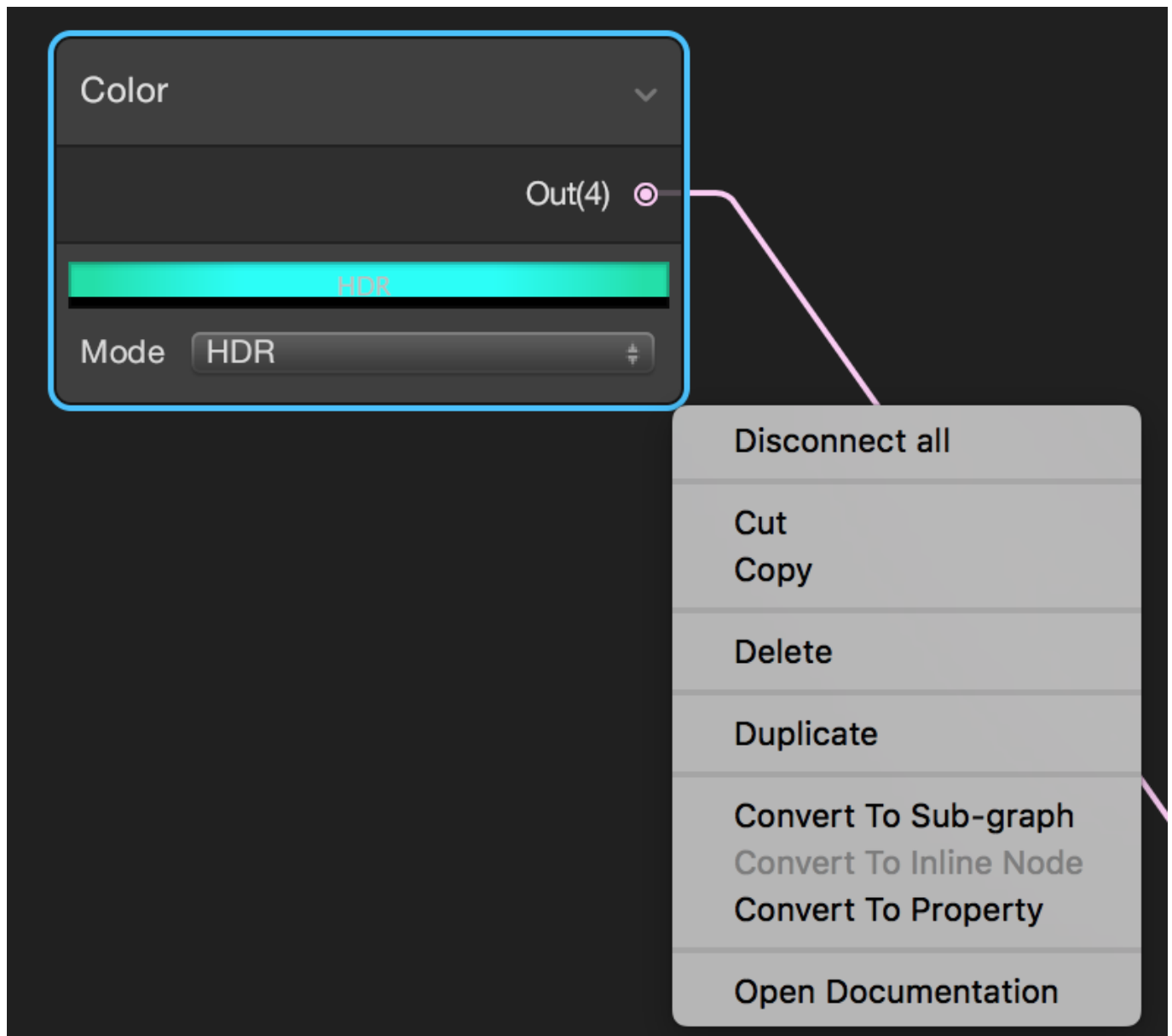
Figure 6-18. Converting an Input node into a property.
