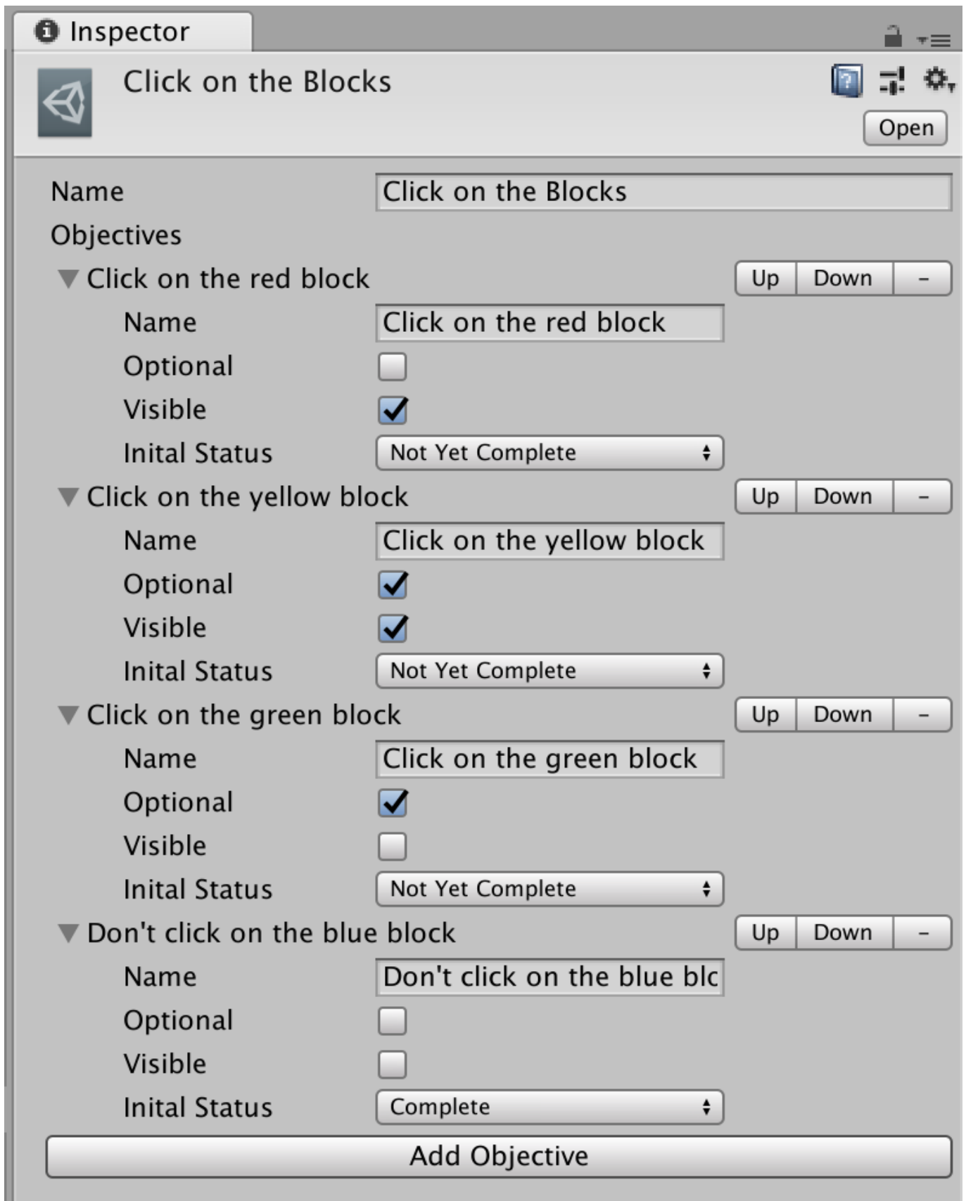
Figure 9-3. The Inspector for the quest asset, with several objectives configured.
