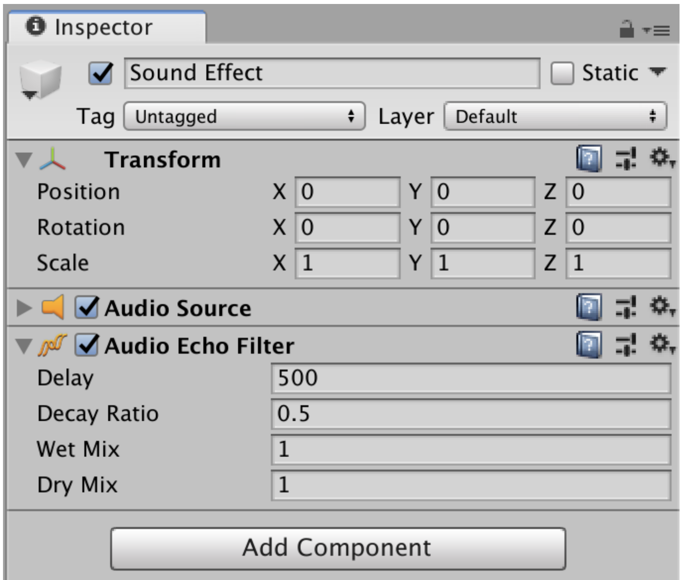
Figure 11-4. An audio effect component, attached to a game object that has an audio source.
