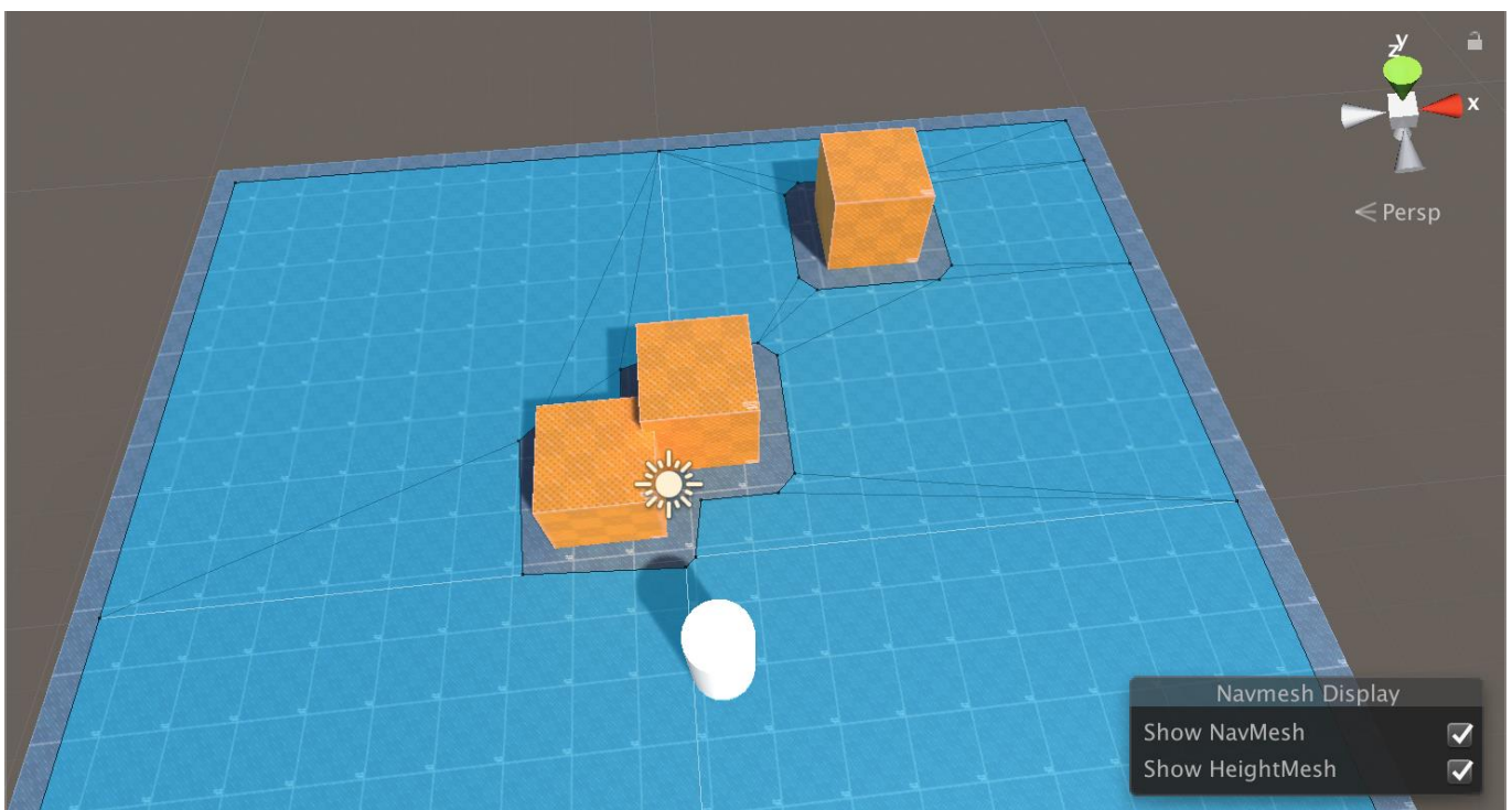
Figure 10-2. A generated navigation mesh. Note how the mesh stops at the edges of the ground, and around the perimeter of the obstacles (which have been marked as Navigation Static).
