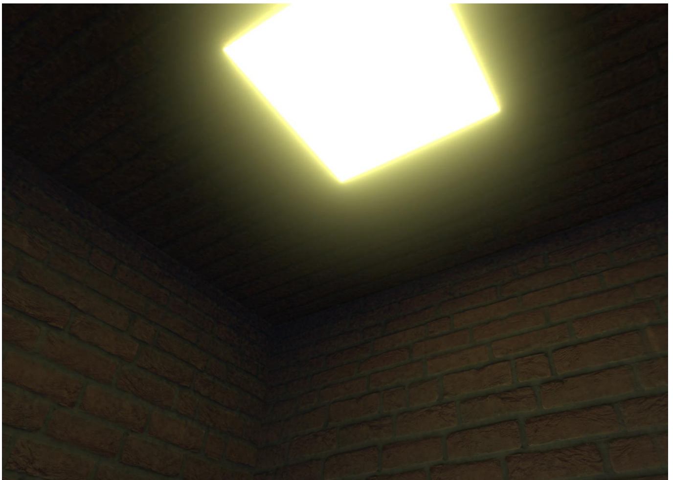
Figure 6-26. Emissive lighting. There are no lights in this scene; instead, the light from the emissive object in the center is illuminating the walls. A bloom effect on the camera completes the effect of a very bright object.
