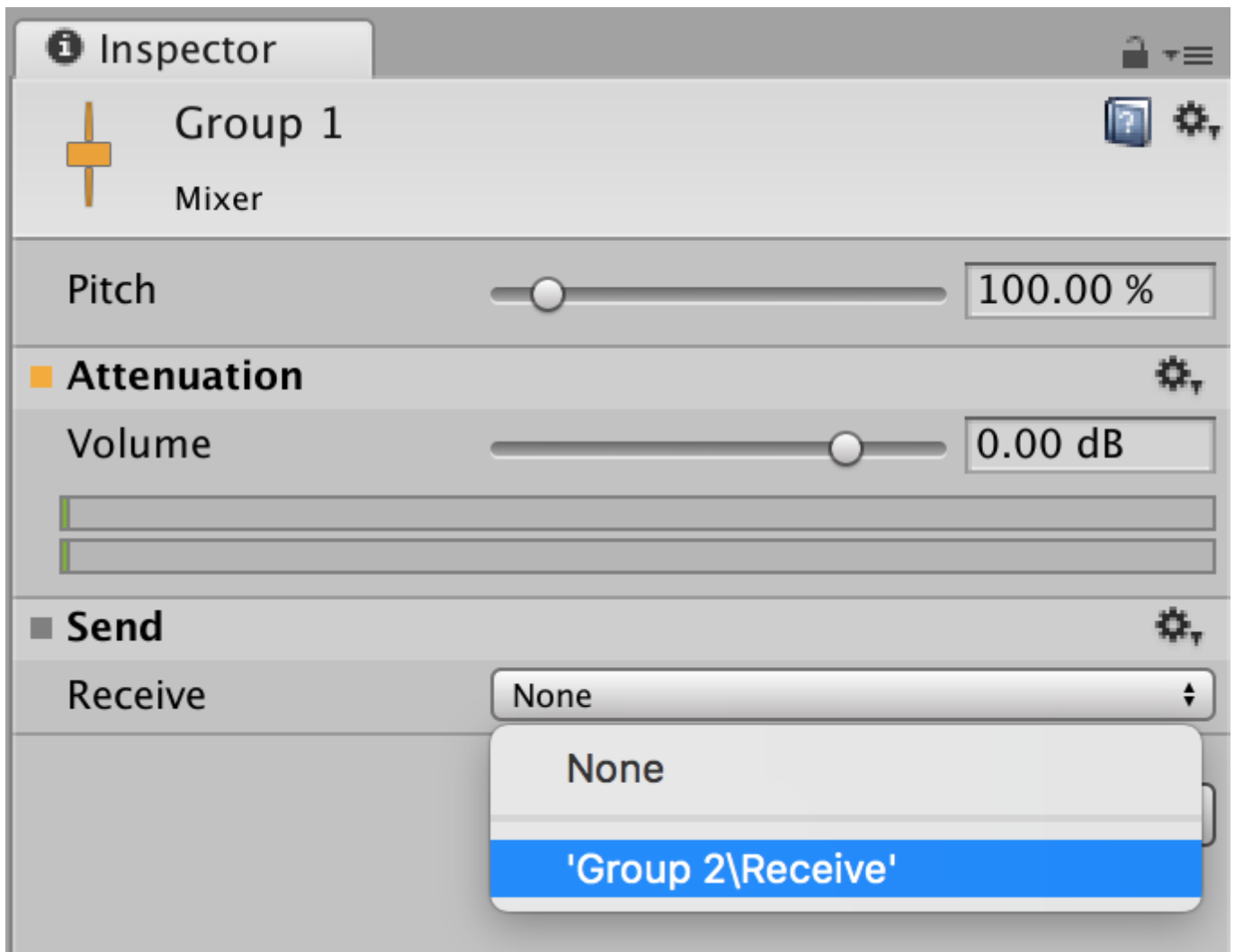
Figure 11-7. Configuring a Send effect to send audio to the specified Receive effect on another group.
