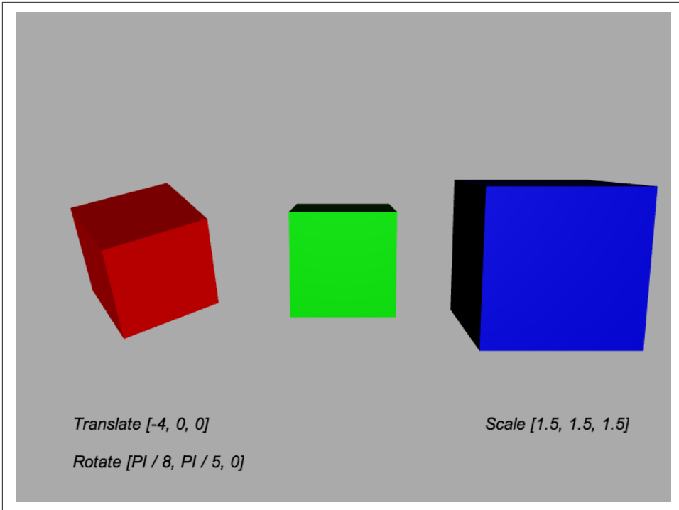
Figure 3-3. 3D Transforms: Translation, Rotation and Scale
