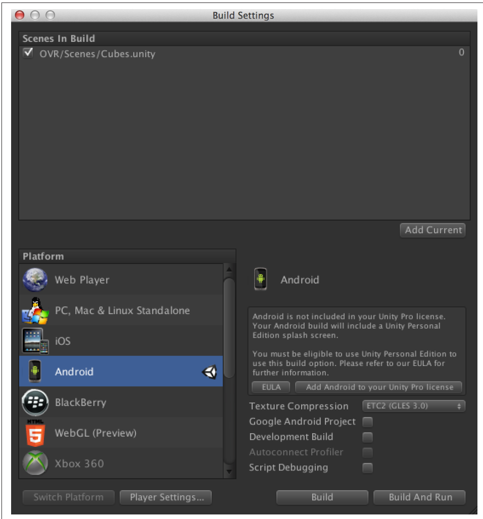
Figure 4-5. Build Settings for the Cube World Android App
