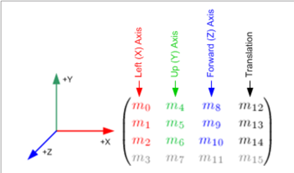
Figure 3-4. A 4x4 Transformation Matrix Defining Translation, Rotation and Scale
