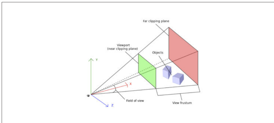
Figure 3-5. Camera, Viewport and Perspective Projection
